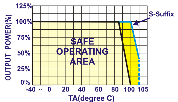
TEMPERATURE DERATING
