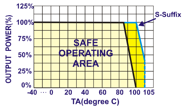
TEMPERATURE DERATING
